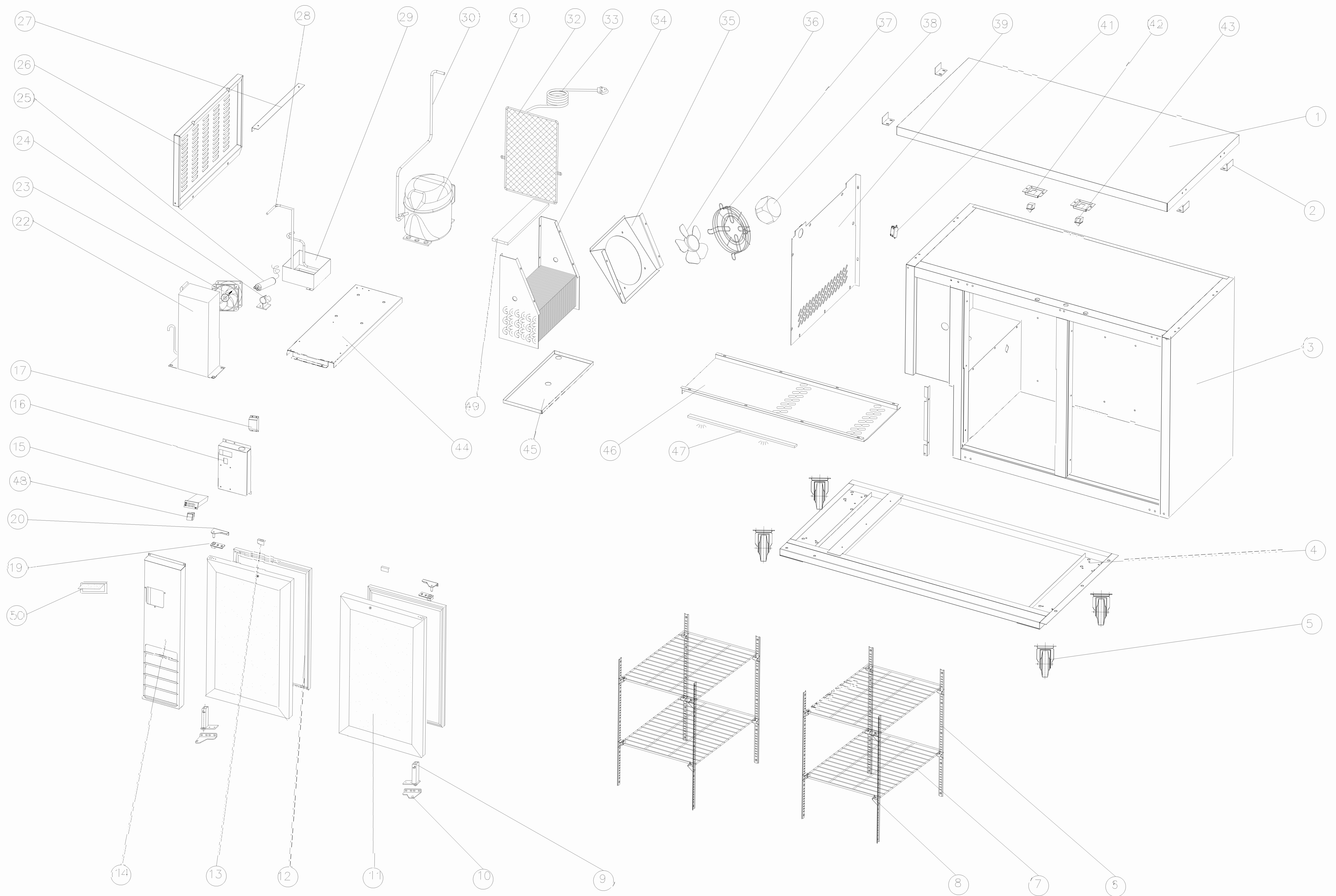
EXPLODE DRAWING OF HC-BC2-24G
