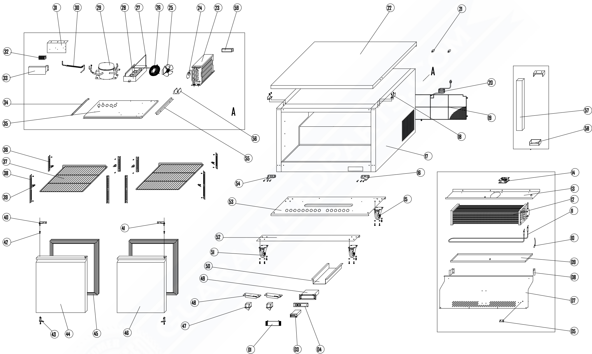
EXPLODE OF HC-TUC36F
