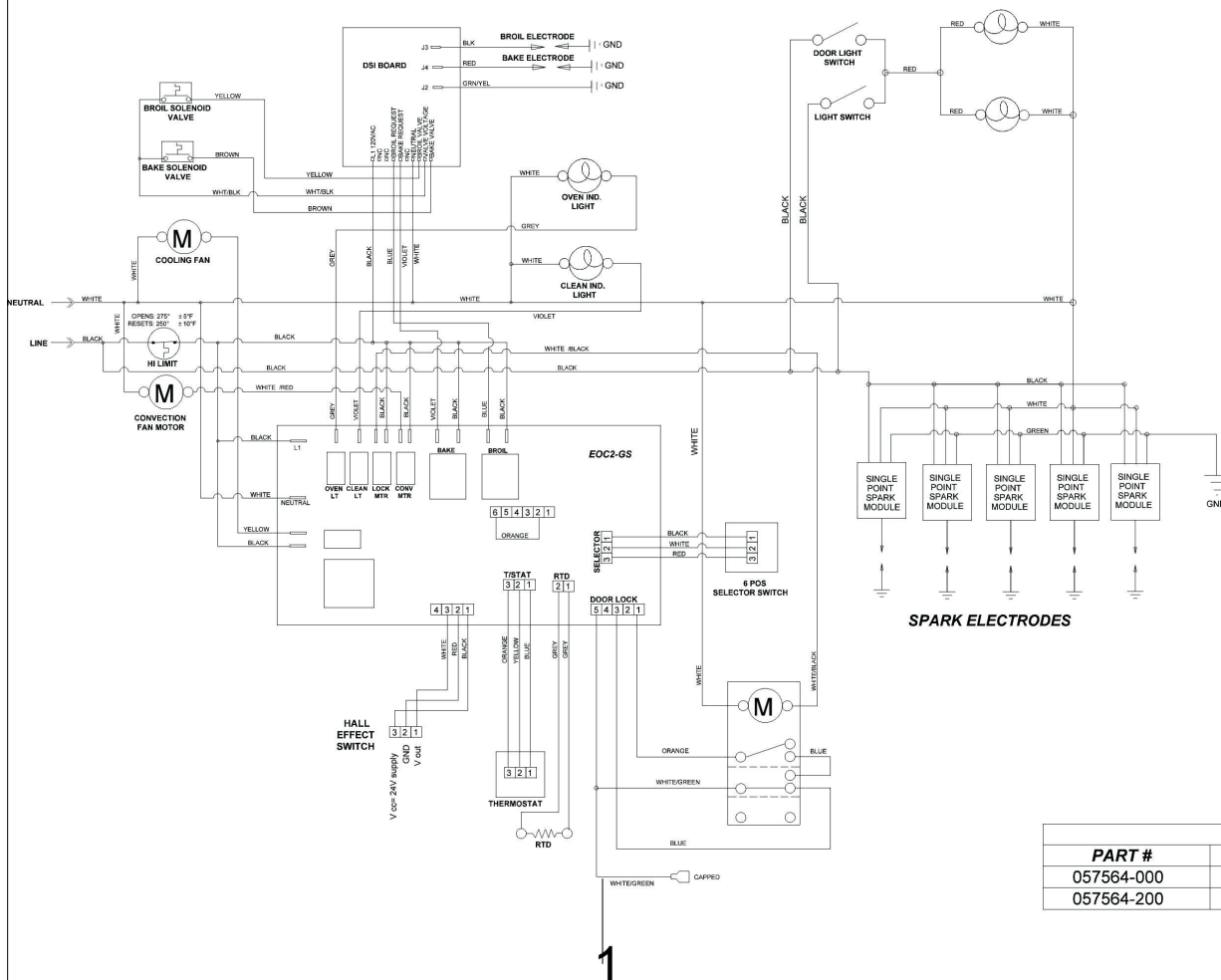
(C)RVGR33025B WIRING DIAGRAM
